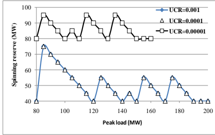
Fig. 4. Amount of spinning reserve associated to case 1.
