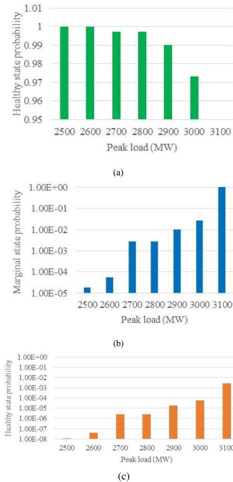
Fig. 16. Probabilities of three states of well-being model of case 3.
