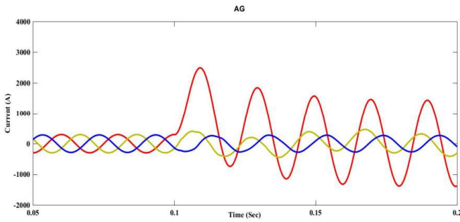
Fig. 7. Line currents waveforms during AG fault, the fault created at t=0.1sec.
