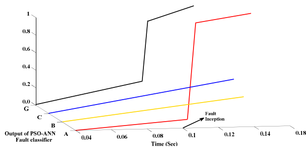
Fig. 17. PSO-ANN classifier output in time domain during AG fault at 25km from sending end with fault resistance 5 \Omega , at t=0.1 sec.
