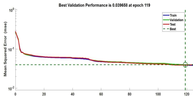
Fig. 19. Convergence characteristics of TLBO-ANN classifier
