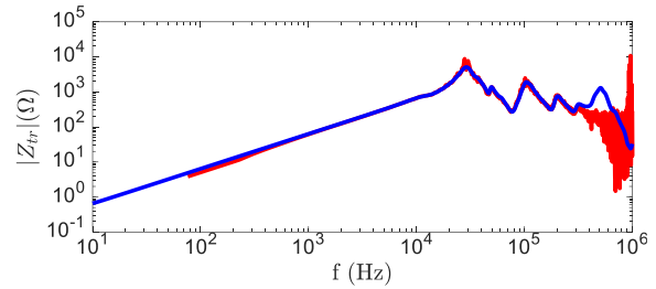
Fig. 14. Comparing the Z_r(j\omega) at the LV side of the transformer, calculated by the LIT result (red) and FRA test result (blue)
