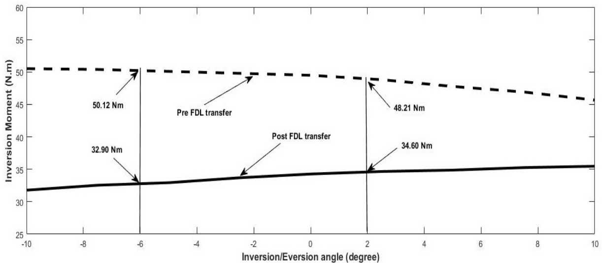
Figure 2. The net isometric inverter moment of subtalar joint muscles before and after the FDL tendon transfer
