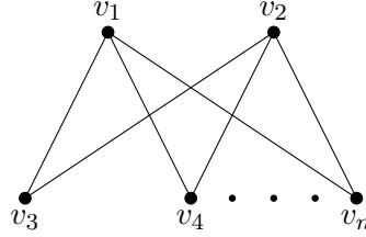
Figure 1: K_{2,n}
