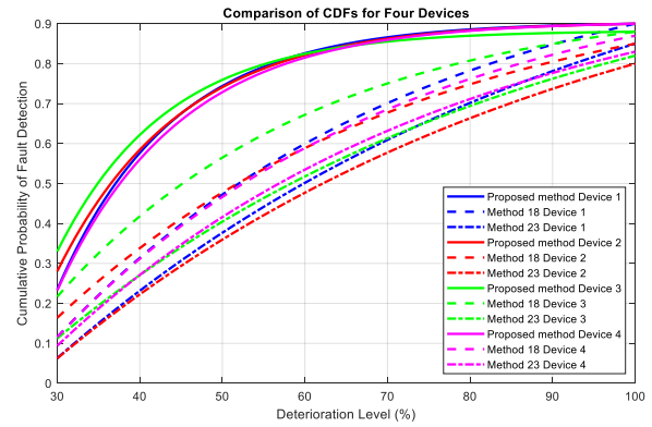
Fig. 9. Comparison of fault detection performance across four devices.
