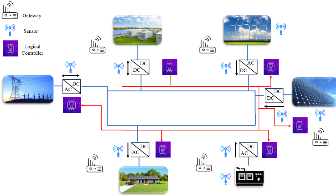
Fig. 1. Energy management and monitoring system.
