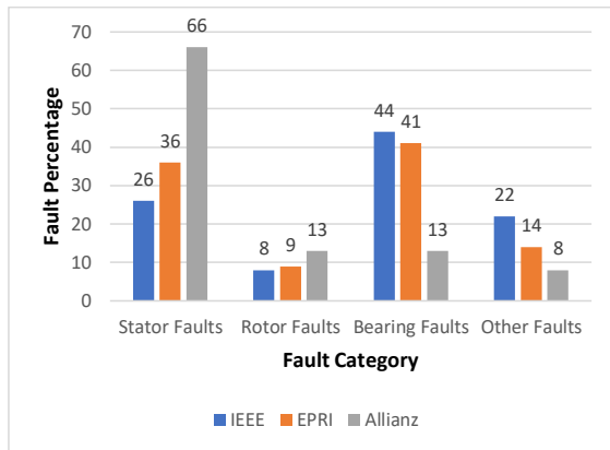
Fig. 1. Percentage of fault distribution.
