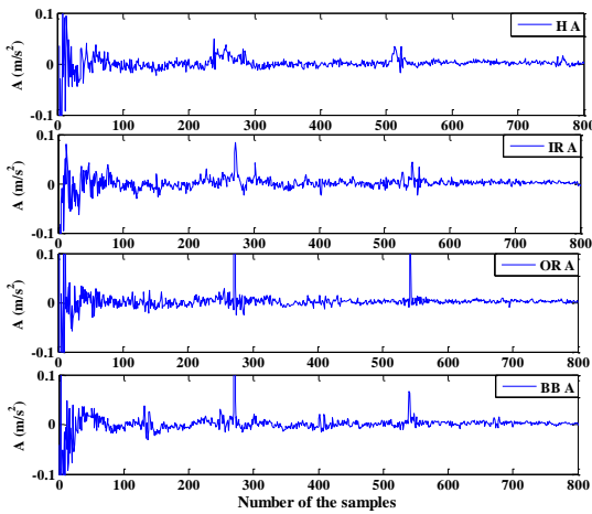
Fig. 8. Axial vibration signals at constant load condition: (H) Healthy, (IR) Inter race, (OR) Outer race, (BB) Ball broken conditions.
