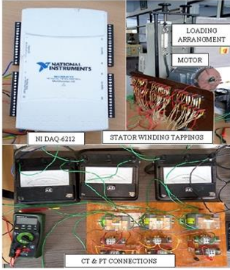
Fig. 3. Original picture of the experimental setup.
