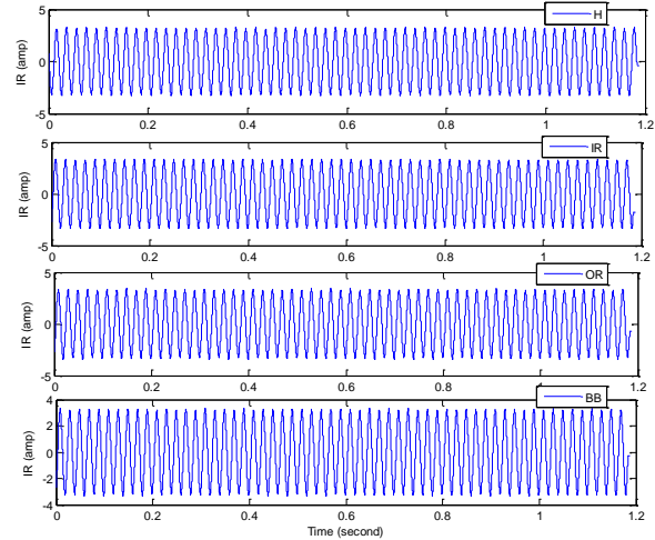
Fig. 6. Current signal at constant load condition: (H) Healthy, (IR) Inter race, (OR) Outer race, (BB) Ball broken conditions.
