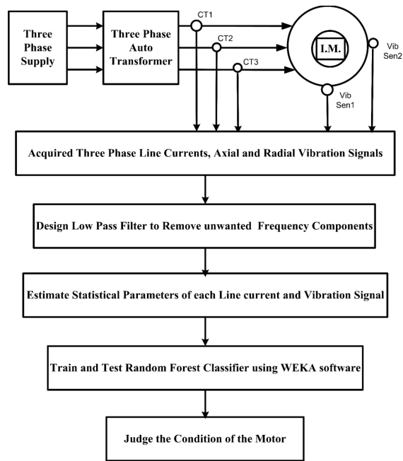
Fig. 5. Flowchart of the proposed scheme.
