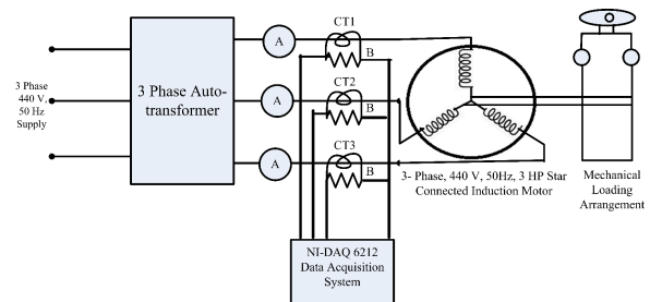
Fig. 2. Schematic diagram of the proposed scheme.
