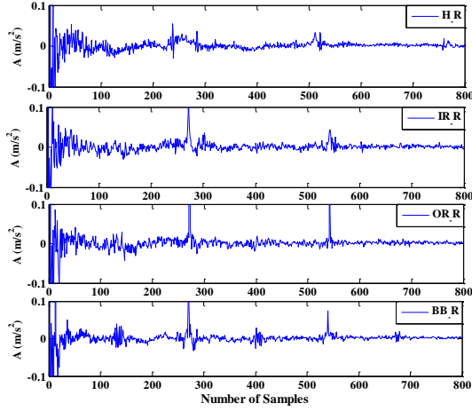
Fig. 7. Radial vibration signals at constant load condition: (H) Healthy, (IR) Inter race, (OR) Outer race, (BB) Ball broken conditions.
