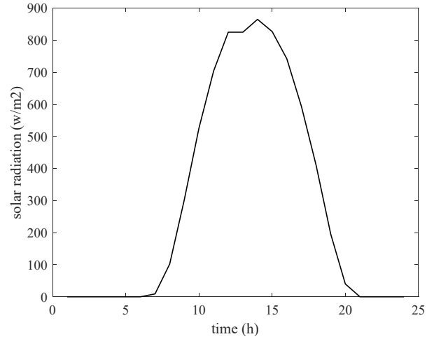
Fig. 10. Hourly solar radiation intensity
