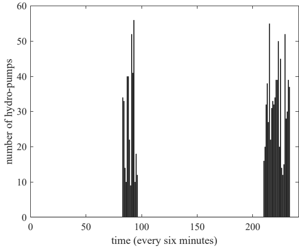
Fig. 7. The optimal number of hydro-pumps at each 6 minutes
