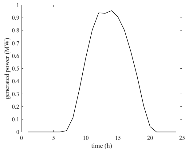
Fig. 12. Hourly generated power of PV unit
