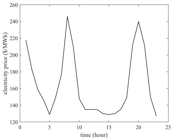
Fig. 13. The hourly electricity price of the main grid [22]
