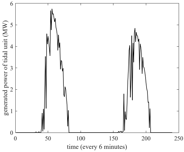
Fig. 8. Generated power of tidal unit with barrage
