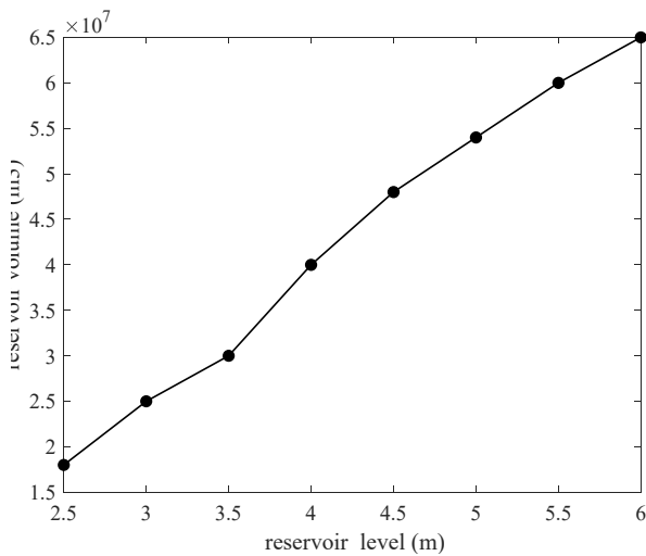
Fig. 4. The volume of the basin considering basin level
