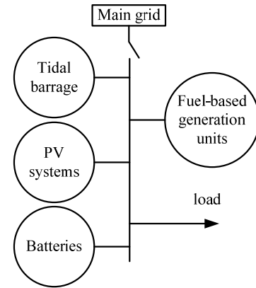
Fig. 1. Topology of understudied microgrid
