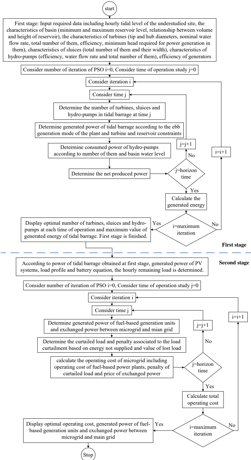
Fig. 2. Flowchart of proposed two-stage method for optimal operation of microgrid
