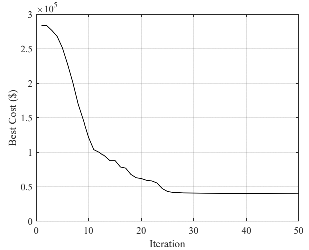
Fig. 14. The convergence of the PSO algorithm
