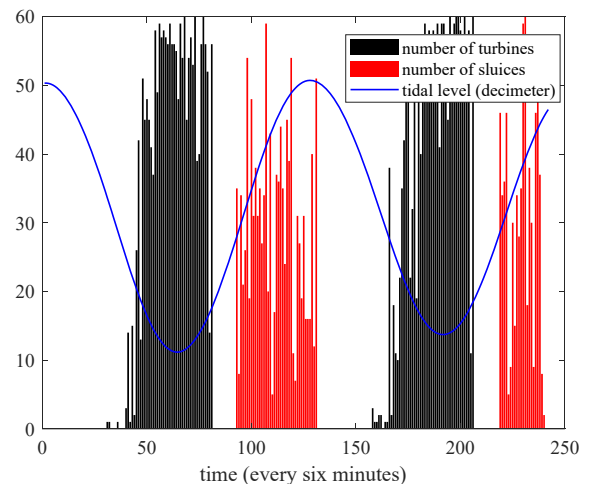
Fig. 6. Optimal number of turbines and gates at every 6 minutes
